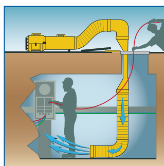
Manhole Entry Device*
